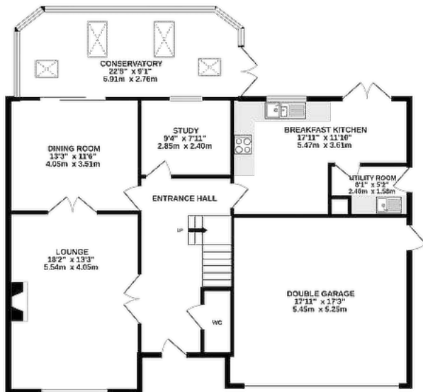
GROUND FLOOR 1354 sq.ft. (125.8 sq.m.) approx.
